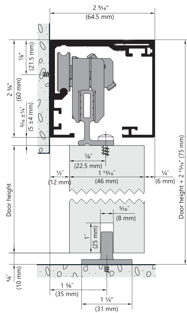
Wall mounting
